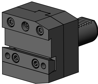
90DEG VDI40 STATIC TOOL OUTPUT: 26mm BLADE COOLANT: EXTERNAL
